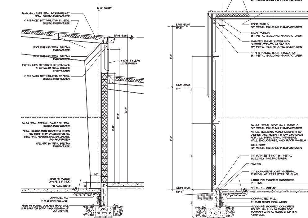
6 WALL SECTION 1/8" = 1'-0" MAIN STORAGE BUILDING
