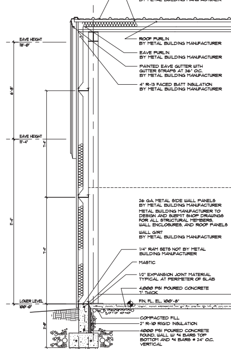
6 WALL SECTION 1/8" = 1'-0" MAIN STORAGE BUILDING
