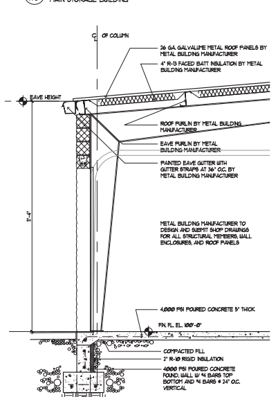
4 WALL SECTION 1/8" = 1'-0" MAIN STORAGE BUILDING
