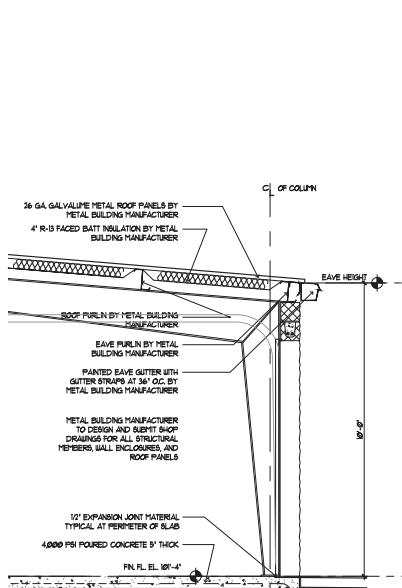
3 WALL SECTION 1/8" = 1'-0" MAIN STORAGE BUILDING
