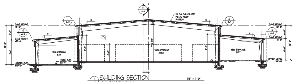
1 BUILDING SECTION 1/8" = 1'-0" MAIN STORAGE BUILDING
