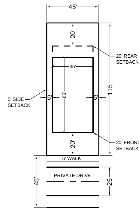
TYPICAL SINGLE FAMILY LOT SCALE: 1" = 50'-0"
