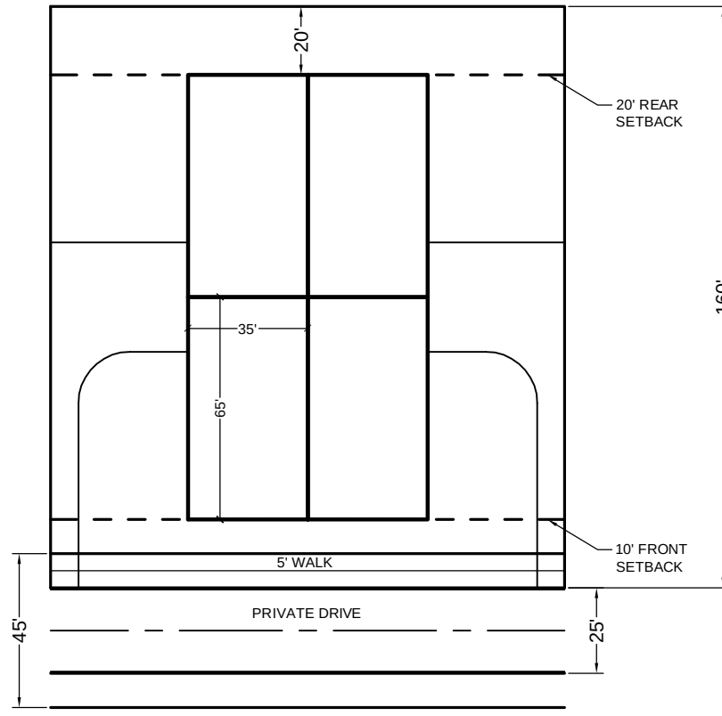
TYPICAL QUAD BUILDING LOT SCALE: 1" = 50'-0"
